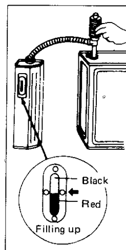
Fill the tank until the red part reaches the arrow mark.
