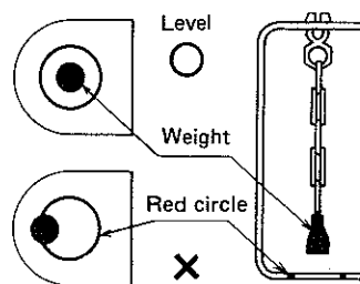
Plumb bob as viewed from above.
